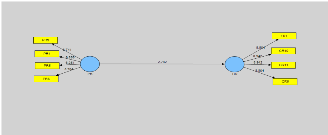
Figure 2 Research Model
